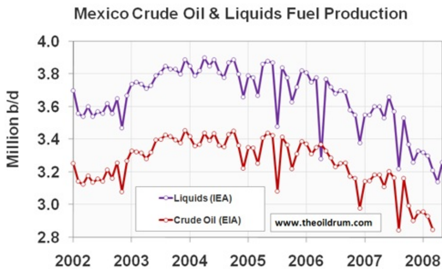
Figure 6 - Mexico Crude Oil & Liquids Fuel Production January 2005 - May 2008
